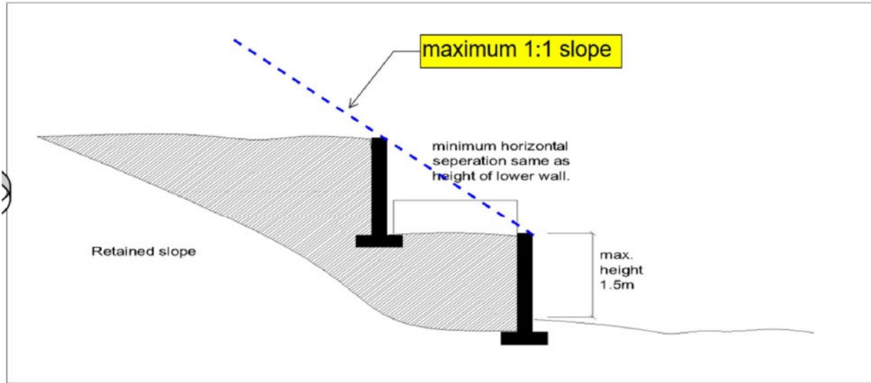
Diagram 8.7: Retaining wall separation
