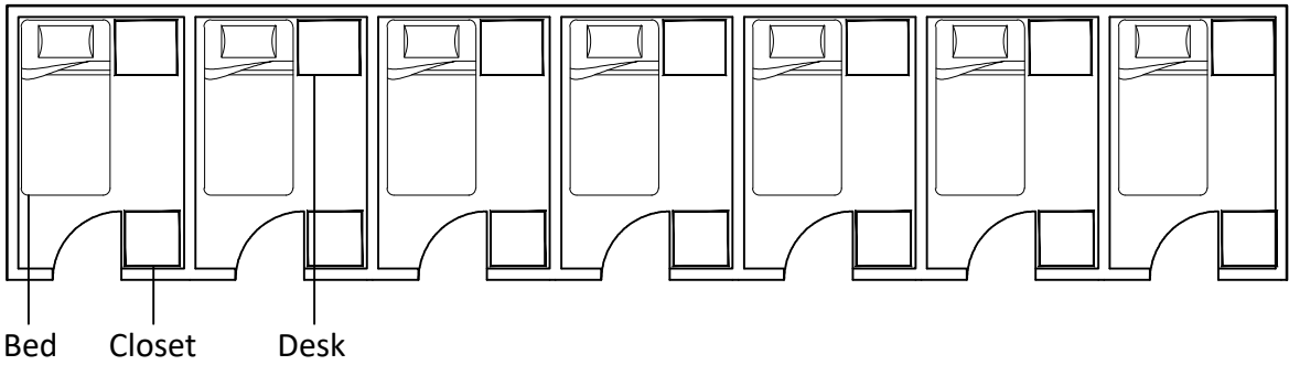
Sleeper Unit (11) 56' x 12' Sq. Ft. :672
