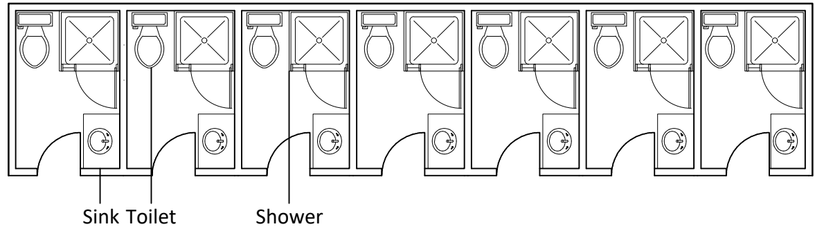
Washroom Unit (2) 56' x 12' Sq. Ft. :672
