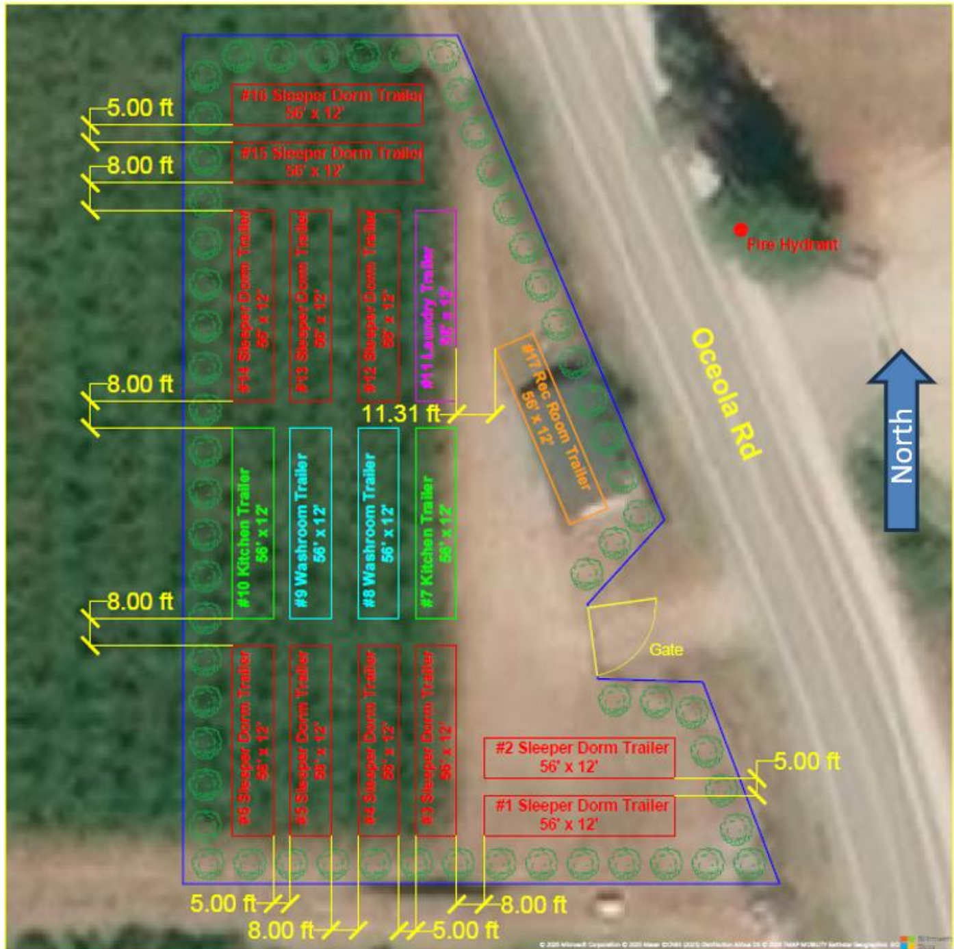
Map 3: Proposed Site Plan
